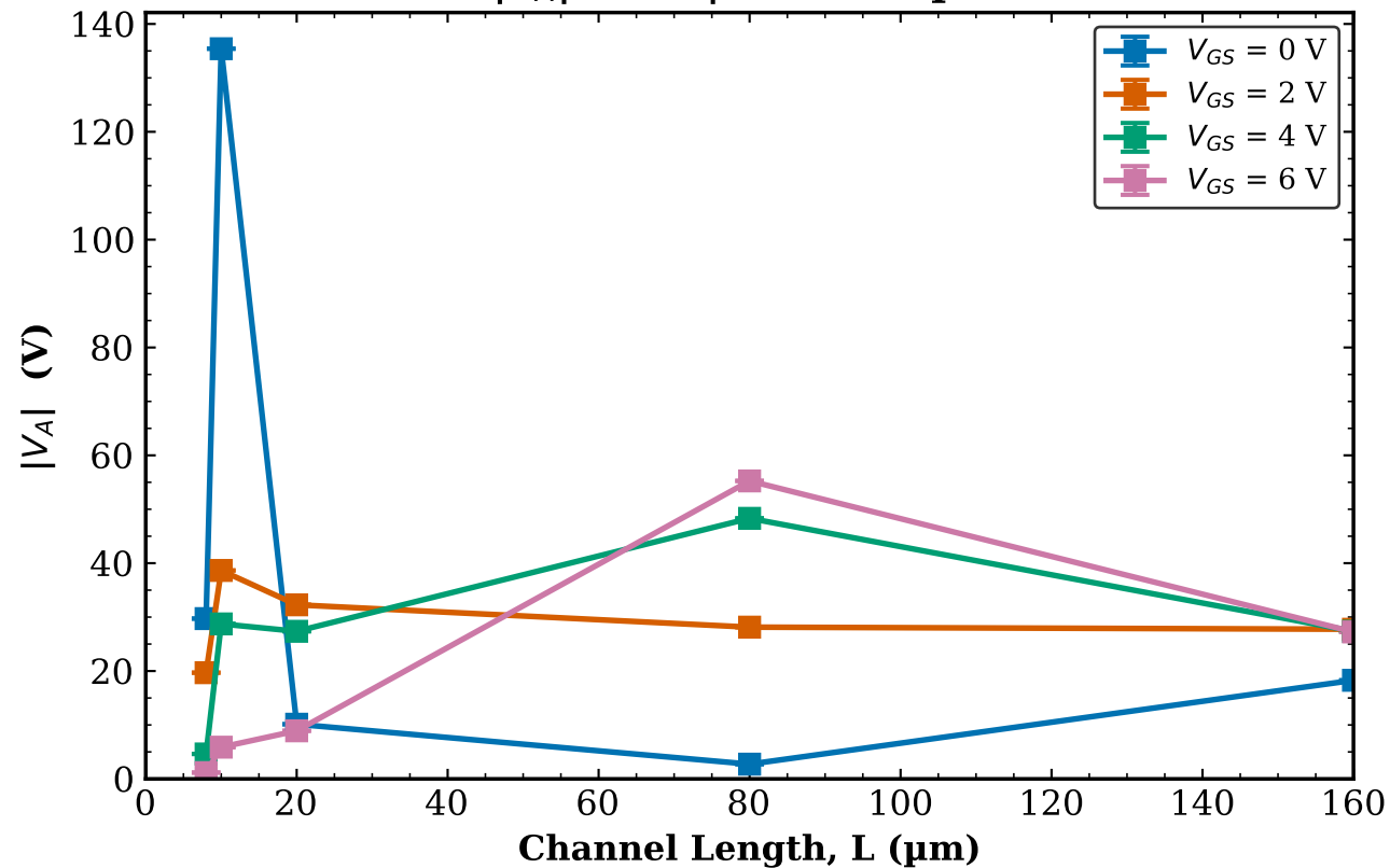
TFT3 Transistor 1 |V_A| vs L | W = 10\text{ }\mu\text{m}
